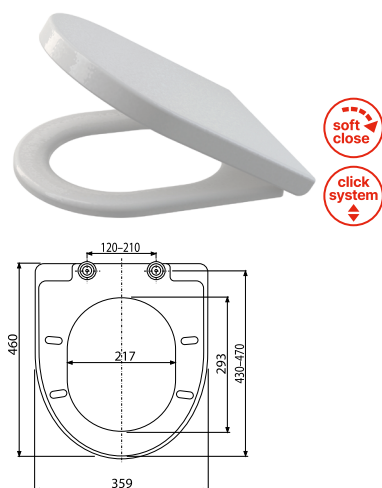
A67 WC seat Softclose, Click system, Duroplast
