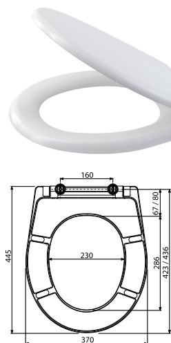
A604 WC seat universal Softclose, Click system, Duroplast
