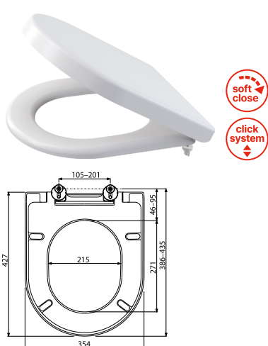
A674S WC seat Softclose, Click system, Duroplast
