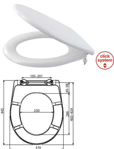
A606 WC seat universal Softclose with integrated insert, Click system, Duroplast
