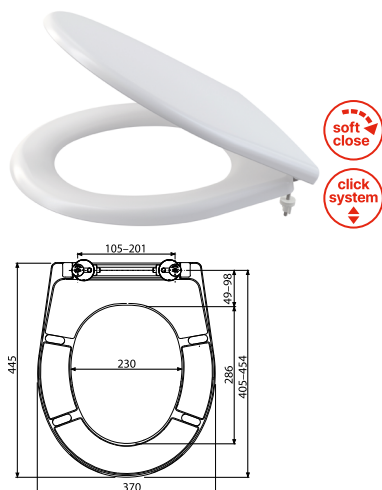
A604 WC seat universal Softclose, Click system, Duroplast
