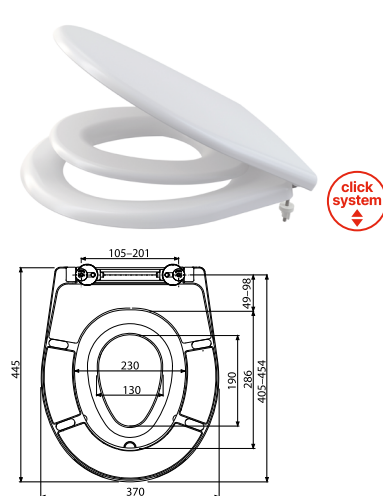
A603 WC seat universal with integrated insert, Click system, Duroplast
